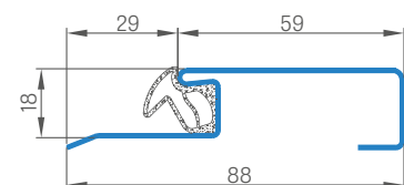
STAINLESS STEEL SHEET THRESHOLD
